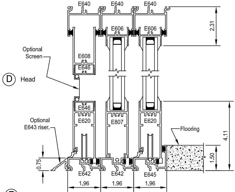
D Head E High Leg Sill
